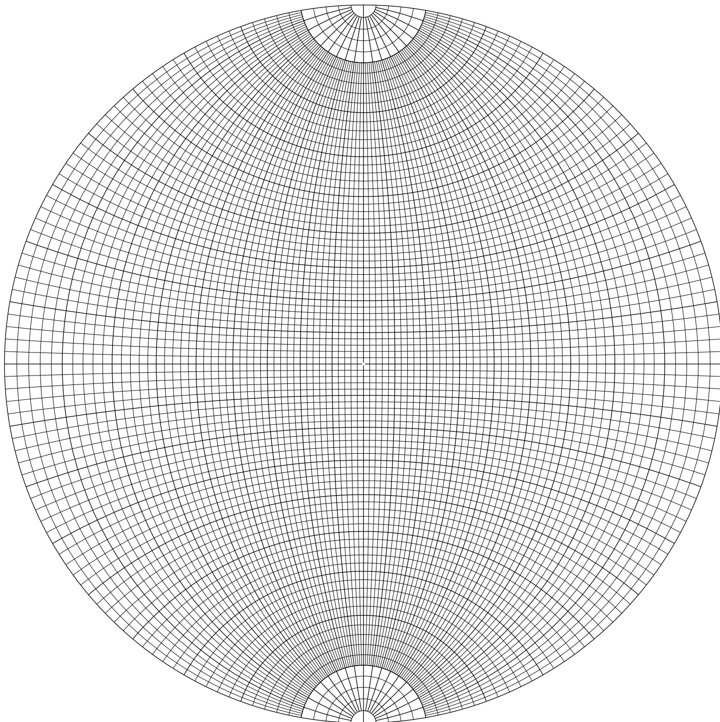
2° Equalangle (Wulff) stereonet © 1996 K.M. Cruikshank
